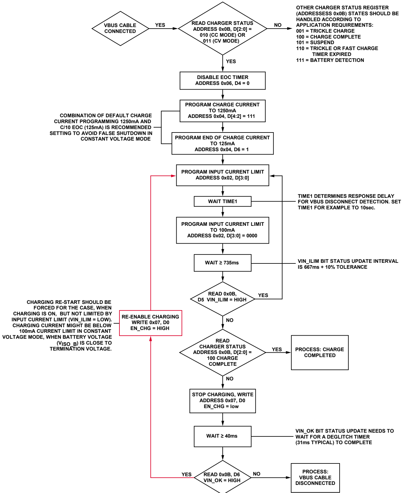
Figure 40. Software Workaround to Detect the Unexpected Mode
