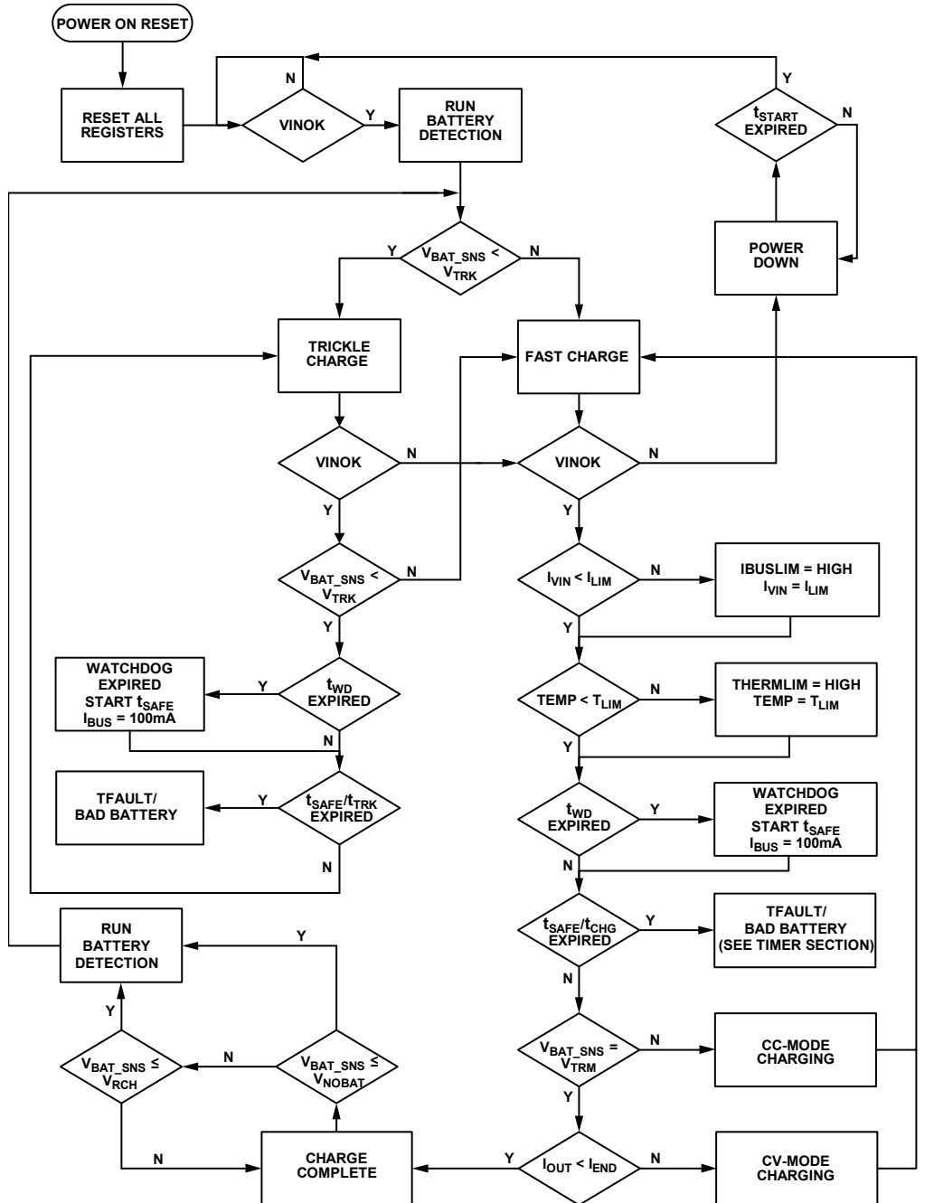
Figure 38. ADP5065 Operational Flowchart
