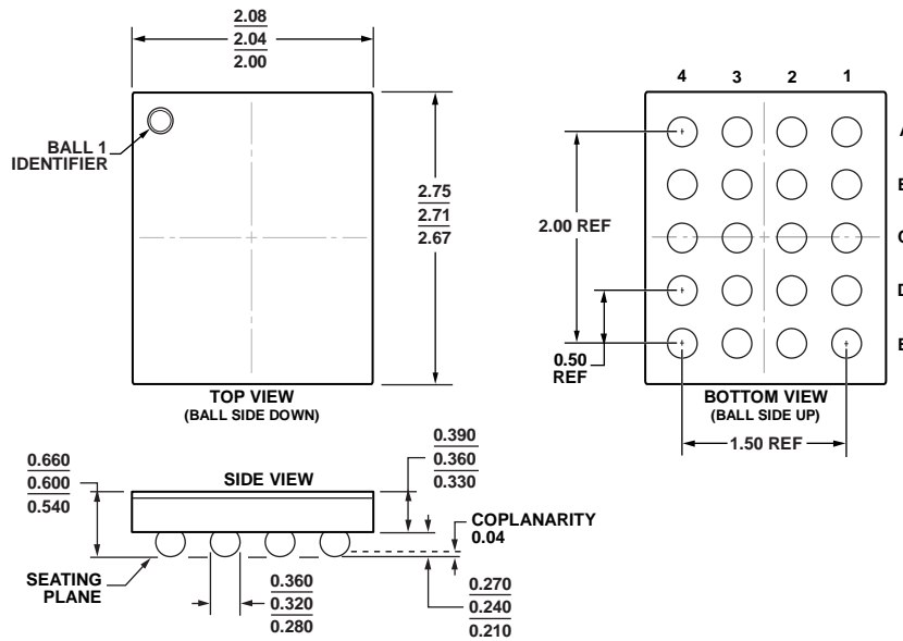
Figure 43. 20-Ball Wafer Level Chip Scale Package [WLCSP] (CB-20-8) Dimensions shown in millimeters
