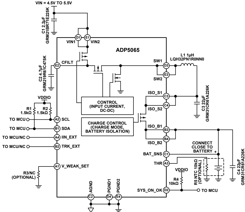
Figure 41. Reference Circuit Diagram
